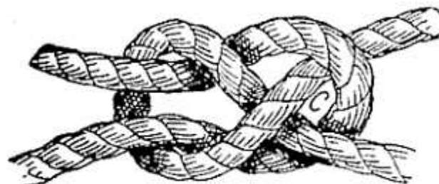
FIG. 22.—Weaver's knot (complete).
