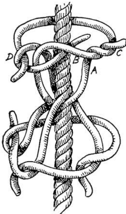
FIG. 118.—Shroud knot (making).
