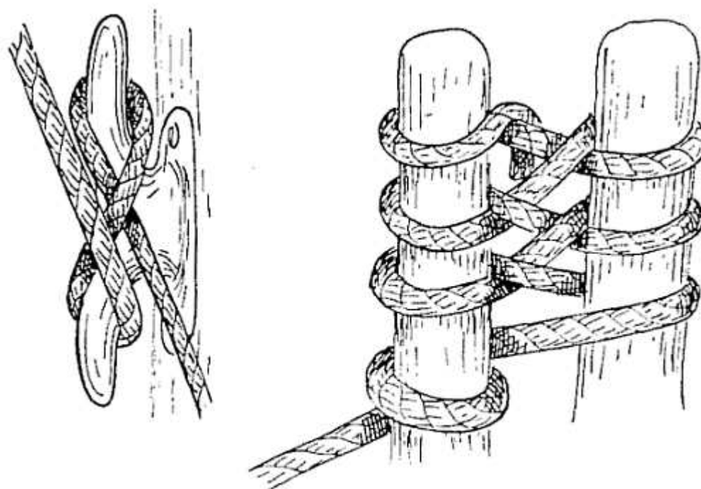
FIG. 57.—Cleat and wharf ties.
