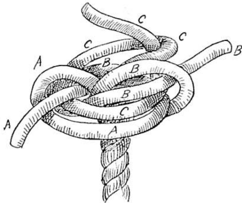
FIG. 132.—Matthew Walker (complete but slack).
