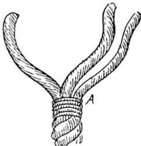
FIG. 104.—Ending rope.
