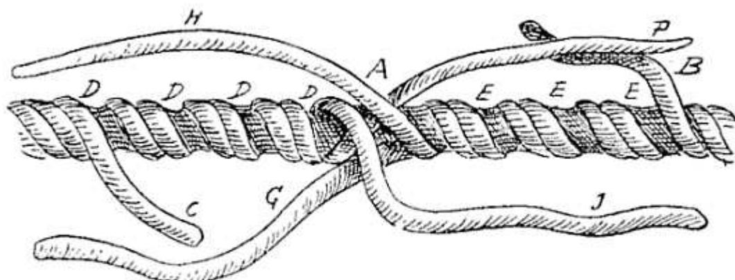
FIG. 107.—Long splice.
