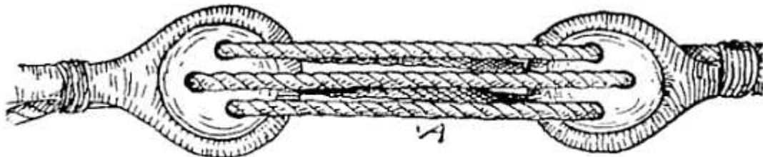
FIG. 98.—Deadeye lashing.
