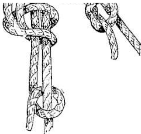
FIG. 56.—Larks' heads and running noose.
