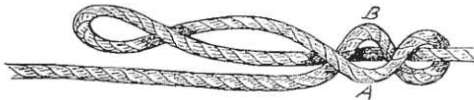
FIG. 70 F.—Monkey chain or single plait (complete).
